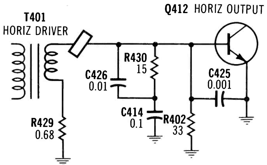
Figure 5. When you notice problems of erratic horizontal linearity or foldover, check the soldered joints at the T401 lugs and all resistors in the base circuit of Q412 horizontal-output transistor.
