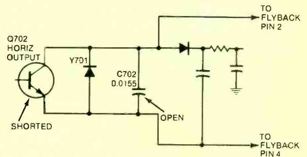
Chassis—General Electric 25YM PHOTOFACT—1780-1
