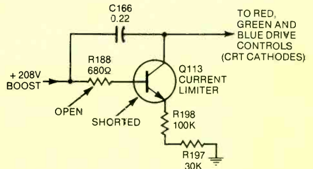
Chassis—General Electric 19JA PHOTOFACT—1328-2
