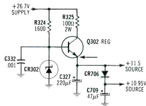
Two dc supply voltages come from the Q302 regulator. Check for a loose soldering joint at the Q302 emitter. It can cause intermittent video or color.
