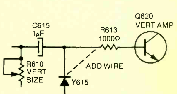
Chassis—General Electric AB (also AC) PHOTOFACT—1904-1
