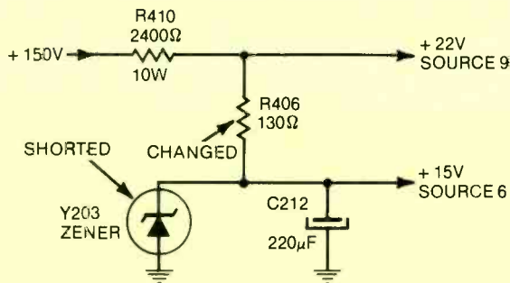
Chassis—General Electric N-2 PHOTOFACT—1219-1
