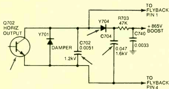
Chassis—General Electric 17YA PHOTOFACT—1578-1
